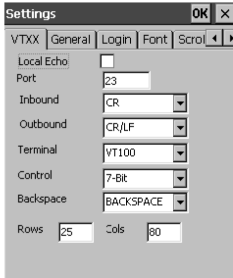
Figure 5-12. The VTXX Settings Dialog Box
