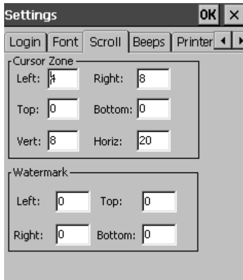
Figure 5-5. The Scroll Settings Dialog Box
